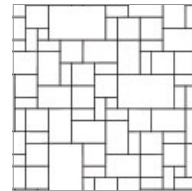
Motif 5 Motif de pose modulaire 16% Citadin M60 (60x163x325) 32% Citadin M60 (60x325x325) 36% Citadin M60 (60x325x488) 15% Supra Citadin M60 (60x488x813)
