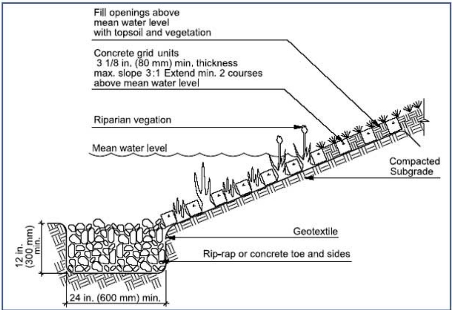
Figure 21. Lake side stabilization with concrete grids
