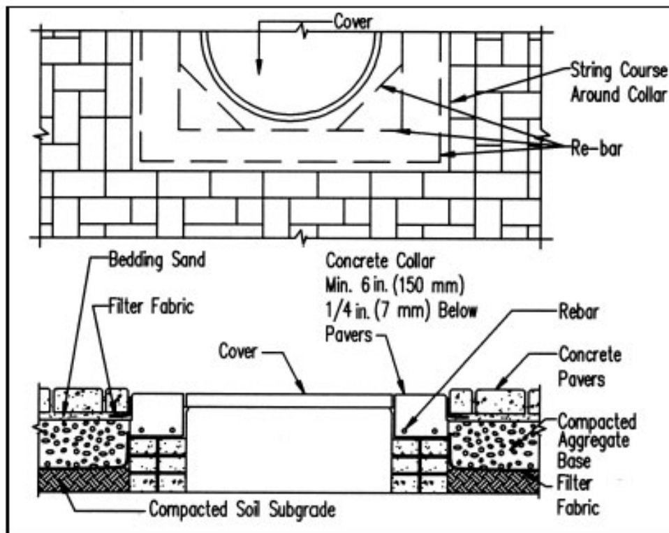
Figure 11. Utility cover.
