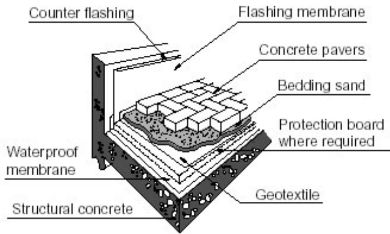
Figure 4. Roof assembly.
